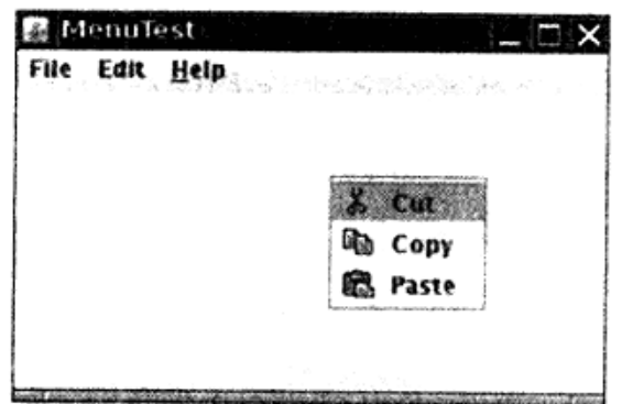
图9-20 弹出菜单
